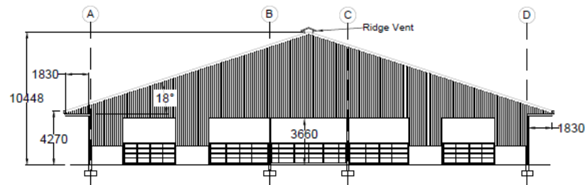
Eastern Elevation
