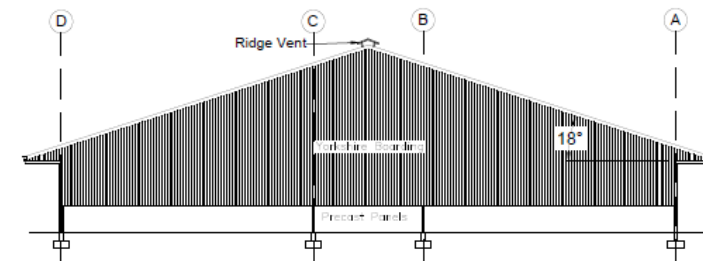
Western Elevation
