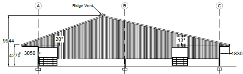
Eastern Elevation
